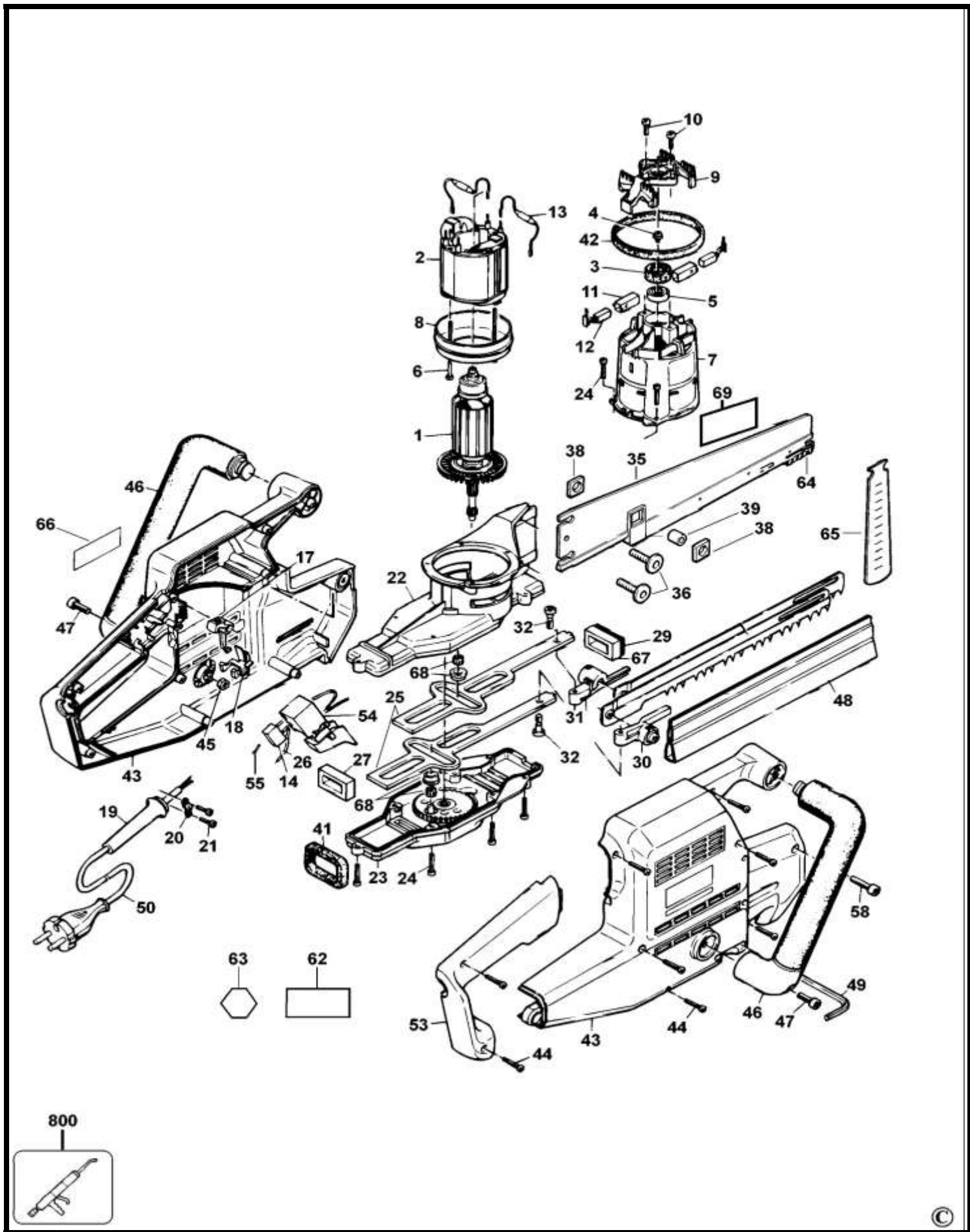
PartsList DW393 UNIVERSALSAW 1
