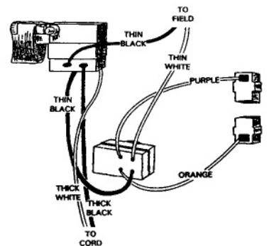
WIRING DIAGRAM
